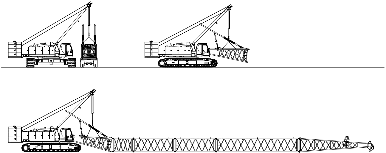
Assembly diagram of boom base
