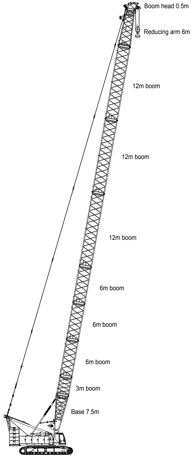
Operating condition of heavy-duty boom
