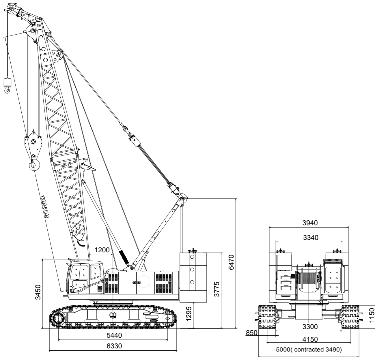
Basic Dimension of the Whole Machine of SCC900E Crawler Crane
