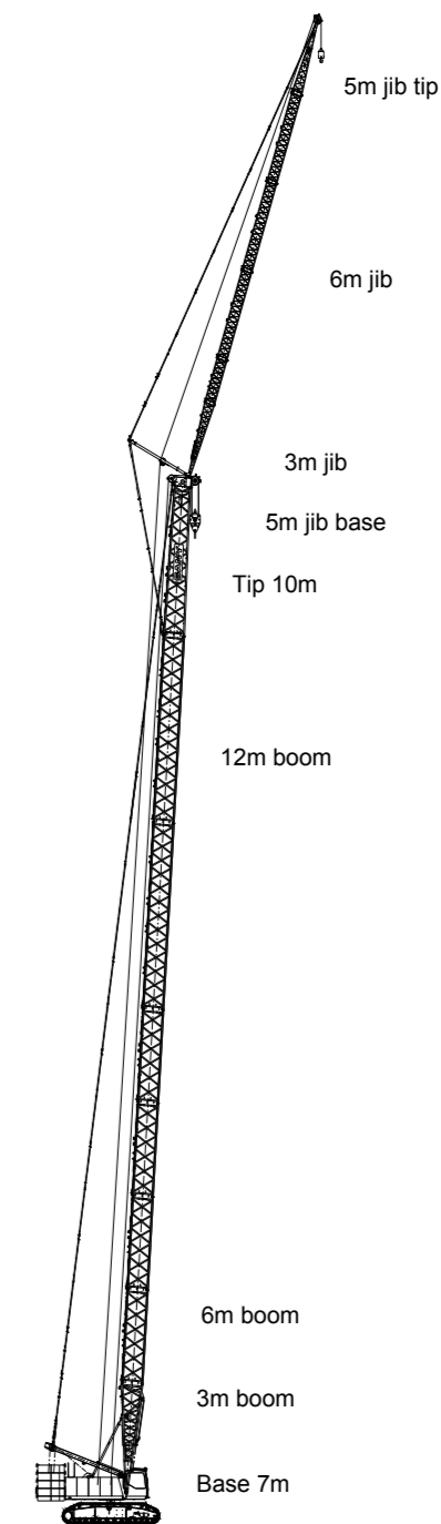
Fixed jib FJ working condition: (17m-71m) + (13m-31m)
